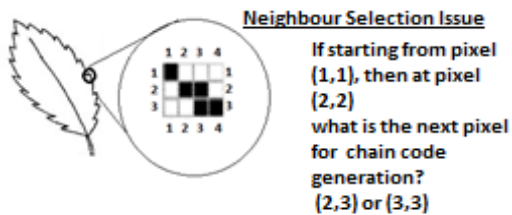
Fig.3. Neighbor selection issue of Freeman chain code with Multi boundary pixels of a leaf.
