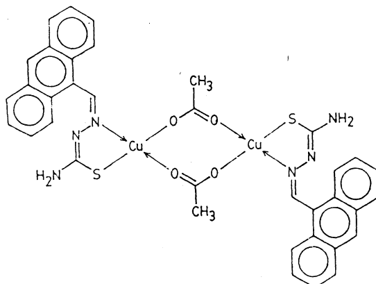
Fig. 1. Structure of Cu(II) chelate, [\text{CuL}(\text{OAc})_2]
